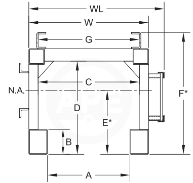
With Pin-up Rail / Auger Rail
